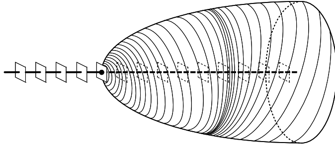
FIGURE 2: A Hopf bifurcation of singularities in a plane field flow.
