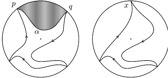
FIG. 4.2. The embedded arc \alpha divides \mathcal{D} (pictured as a smooth disc) into two discs, one of which is collapsed to a point x .
