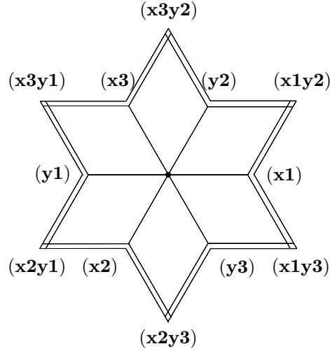
FIG. 4.1. The six pairs of contiguous edges in \partial\mathcal{D} each corresponds to a configuration where one AGV is docked at an extreme vertex of the graph. Outermost vertices of \partial\mathcal{D} are points where both AGV's are docked. Labelling the edges (x_i) and (y_j) and the vertices (x_iy_j) yields the cyclically ordered grammar \mathcal{G} .
