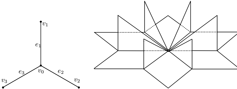
FIG. 3.1. [left] The Y-graph \Upsilon ; [right] the configuration space \mathcal{C} embedded in R^3 .
