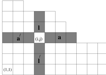
Figure 10.3 The arm a , coarm a' , leg l and coleg l' of a cell.
