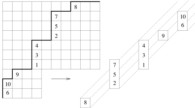
Figure 10.7 A SYT in the LLT product of vertical strips (1^3/1^2, 1^4/1, 1^3, 1^2/1, 1^2) with 5 inversion pairs.
