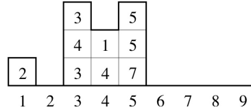
Figure 10.14 A nonattacking filling of (1, 0, 3, 2, 3, 0, 0, 0, 0)' .
