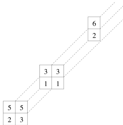
Figure 10.6 A tuple of SSYT occurring in the definition of an LLT product of the shapes (22, 22, 11) . This tuple has 13 inversion pairs.
