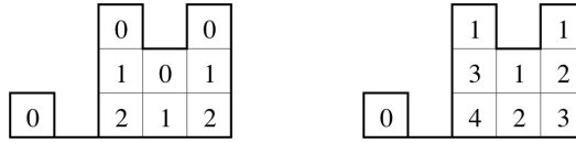
Figure 10.13 The leg lengths (on the left) and the arm lengths (on the right) for (1, 0, 3, 2, 3, 0, 0, 0)' .
