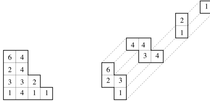
Figure 10.10 On the left, a filling \sigma , and on the right, the term \mathbf{T}(\sigma) in the corresponding LLT product of ribbons.
