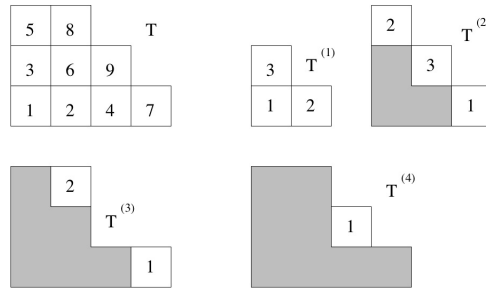
Figure 10.4 The (3, 3, 2, 1)-sections of a SYT.
