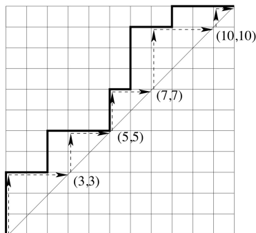
Figure 10.15 The bounce path (dotted line) for a Dyck path.
