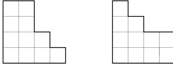
Figure 10.1 On the left, the Ferrers graph of the partition (4, 3, 2, 2) , and on the right, that of its conjugate (4, 3, 2, 2)' = (4, 4, 2, 1) .
