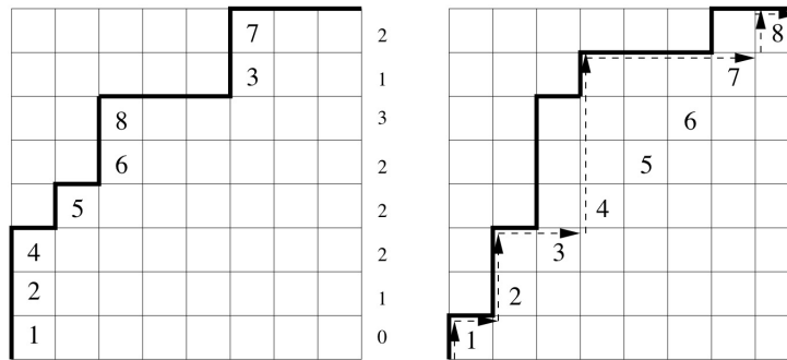
Figure 10.16 On the left, a Dyck path \pi , and on the right, \zeta(\pi) , together with its bounce path.
