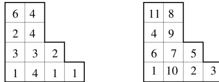
Figure 10.9 On the left, a filling of (4, 3, 2, 2) with reading word 64243321411 and on the right, its standardization.
