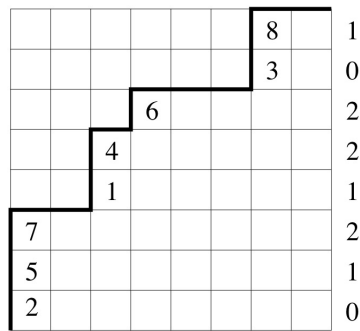
Figure 10.5 A parking function with \text{area} = 9 , \text{dinv} = 6 , and reading word 64781532.
