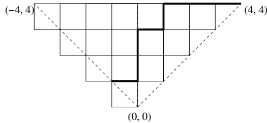
Figure 5: A shifted Dyck path in \mathcal{E}_4 with area = 6
