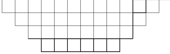
Figure 10: Path last touching diagonal at (1, 1) .
