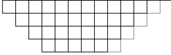
Figure 9: Path never touch y = x except the endpoint.
