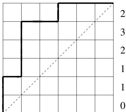
Figure 1: A Dyck path, with row lengths on the right. The area statistic is 1 + 1 + 2 + 3 + 2 = 9 .
