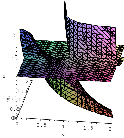
Figure 14: the pole variety of the cube grove generating function
