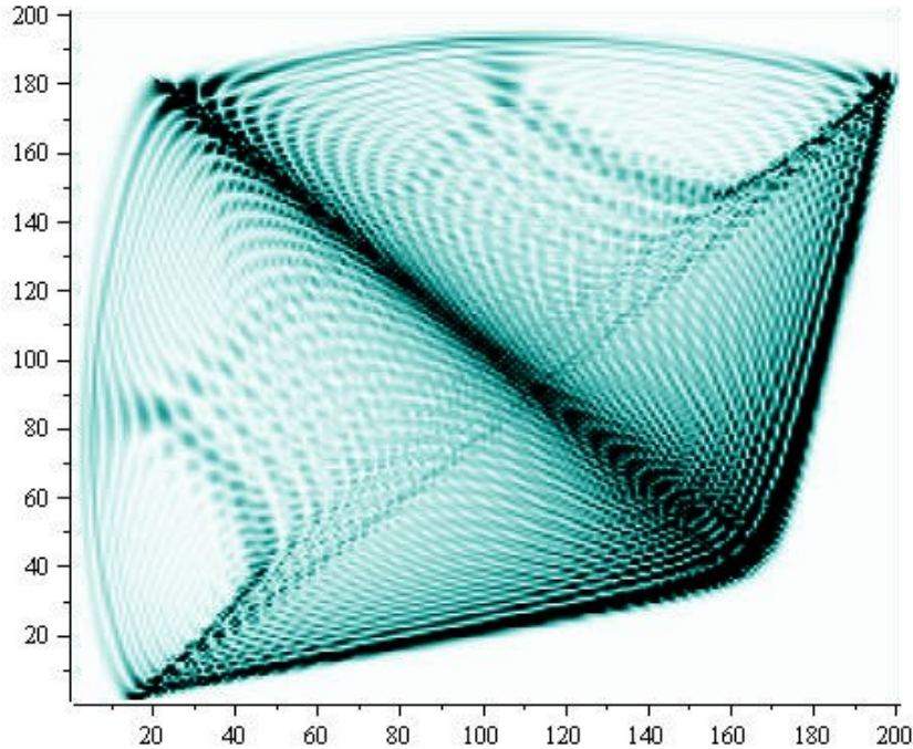
Figure 16: Intensity plot of amplitudes at time 200 for a typical quantum walk
