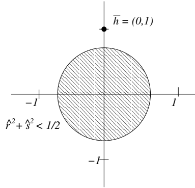
Figure 10: the disk B_2^* and the point \tilde{h} ; the region U is the interior of the convex hull of B_2^* \cup \tilde{h} , minus the boundary of B_2^*
