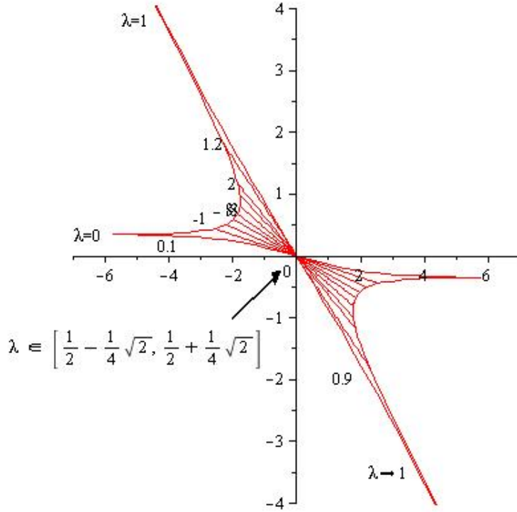
Figure 7: the amoeba for F = 1 - (1 - X)Y/\sqrt{2} - XY^2
