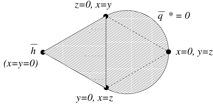
Figure 15: the dual cone in symmetrized coordinates
