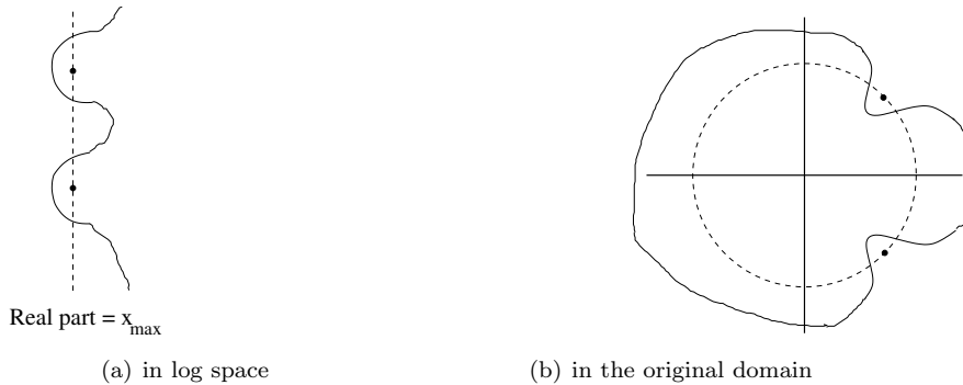
Figure 2: the localizing chain, in logarithmic and original coordinates
