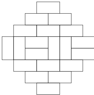
Figure 9: the Aztec diamond of order 4, tiled by dominoes
