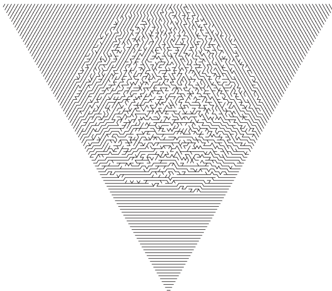
Figure 13: a random cube grove of size 100
