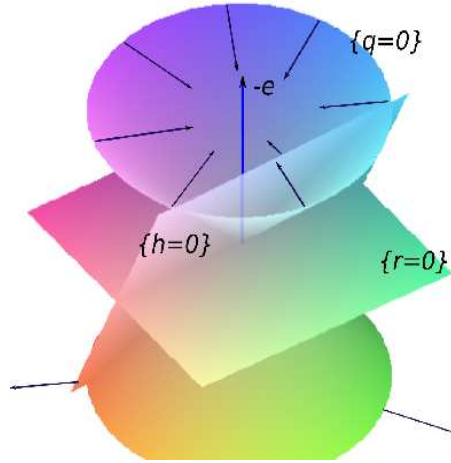
Figure 18: the vector field \tilde{\eta}
