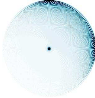
Figure 17: two-dimensional Hadamard QRW probability amplitudes at time t = 200
