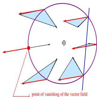
Figure 21: showing where the homotopy intersects the quadric
