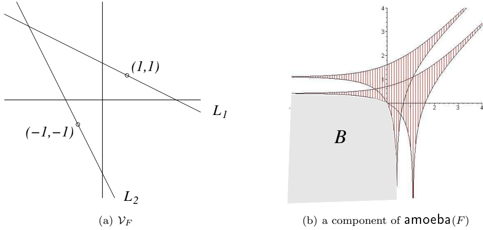
Figure 6: the zero set of (3 - X - 2Y)(3 + 2X + Y) from example 2.19 and the OPS component
