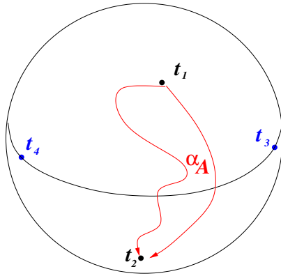
Figure 20: the topological sphere \overline{\mathcal{V}_{\tilde{q}}} , its real part (the equator) and its intersections with the planes \{\tilde{h} = 0\} and \overline{X_{\mathbf{r}}}
