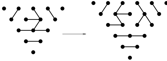
Figure 12: an order 4 cube grove, shuffled to become an order 5 grove
