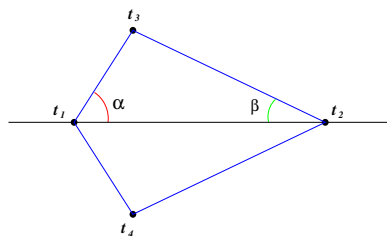
Figure 22: the logarithm as an arctangent
