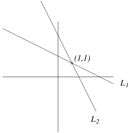
Figure 5: the zero set of the function L_1L_2 := (3 - X - 2Y)(3 - 2X - Y)
