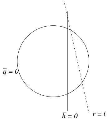
Figure 19: when \mathbf{r} is outside B_2^*
