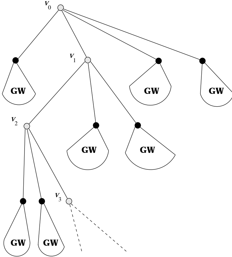
Figure 1. Schematic representation of size-biased Galton-Watson trees.
