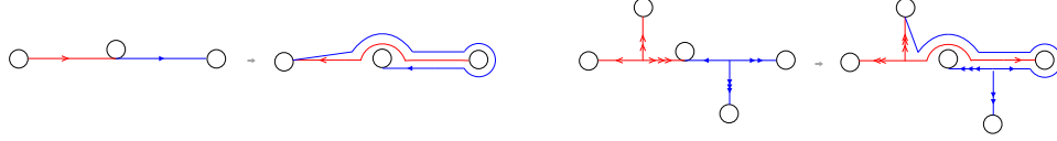
Figure 10. g_{(1,1)} [left]; g_{(2,2)} [right].
