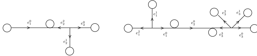
Figure 8. G_{(1,2)} [left]; G_{(2,1,3)} [right].
