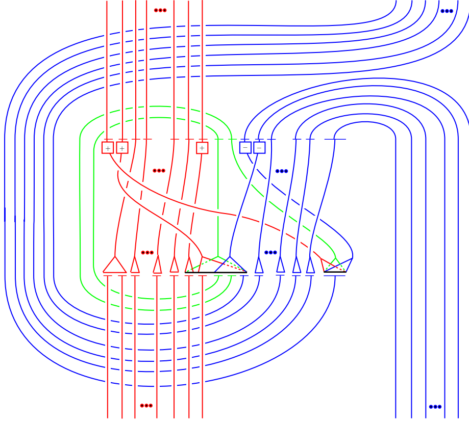
Figure 15. The fundamental domain of U_{(p,q)}^m , cf. Fig. 4.
