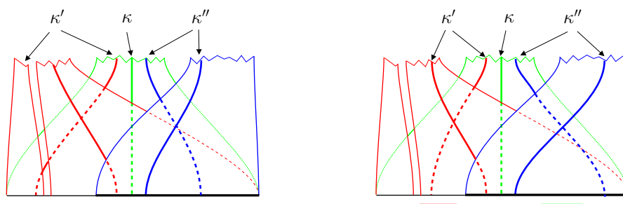
Figure 20. A closeup of the branch line in the proof of Main Theorem (b); p and q even [left]; p and q odd [right].
