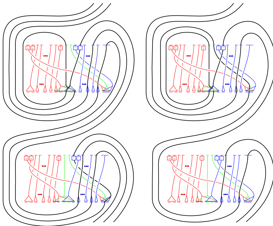
Figure 19. The orbit \kappa'' in Main Theorem (b): q is odd [left]; even [right].
