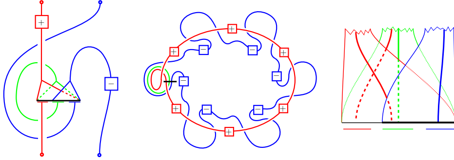
Figure 17. A cartoon representation of the fundamental domain of \mathcal{U}_{(1,1)}^m [left]; the unknots \kappa , \kappa' , and \kappa'' in the case m = 6 [center]; all three orbits pass through the same branch line [right].
