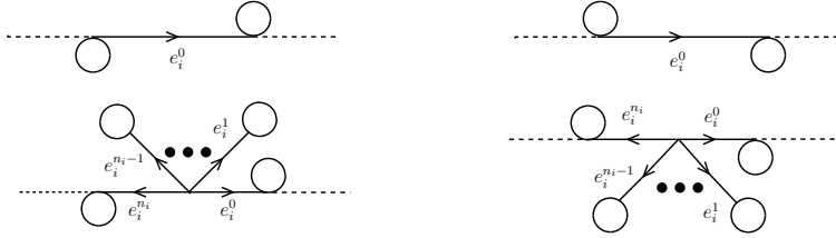
Figure 7. i odd, n_i = 1 [upper left]; i even, n_i = 1 [upper right]; i odd, n_i > 1 [lower left]; i even, n_i > 1 [lower right].
