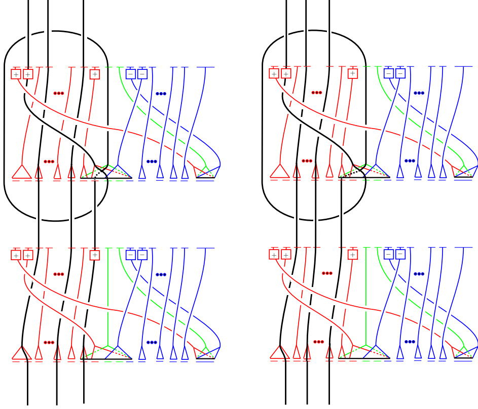
Figure 18. The orbit \kappa' in Main Theorem (b); p is odd [left]; even [right].
