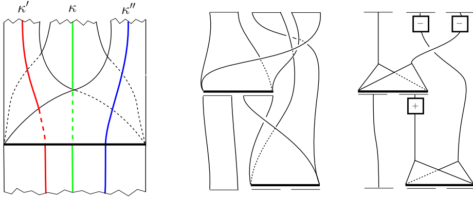
Figure 3. \kappa', \kappa, \kappa'' from left to right [left]; a template and its cartoon representation — top and bottom are identified [center, right].
