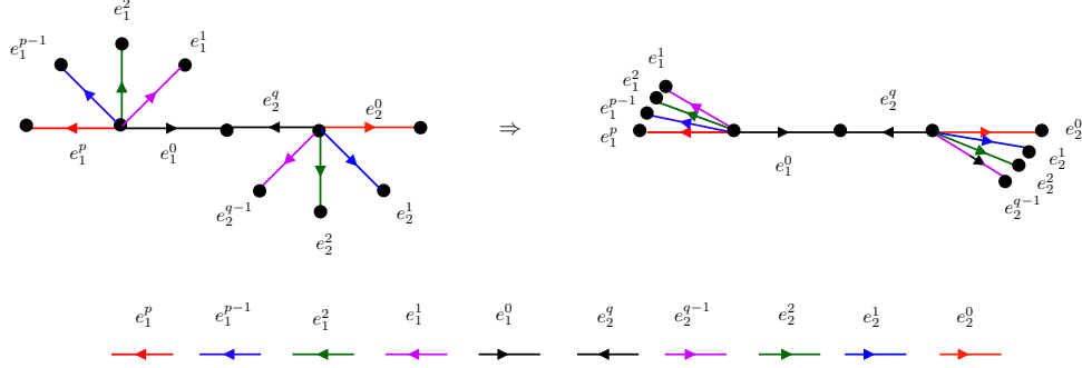
Figure 11. Flattening a pair of stars into strips.
