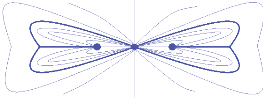
Figure 4.12: Separating trajectories (solid) and generic trajectories (transparent), for the quadratic differential from equation 4.2.1. The three blue circles are the double poles.
