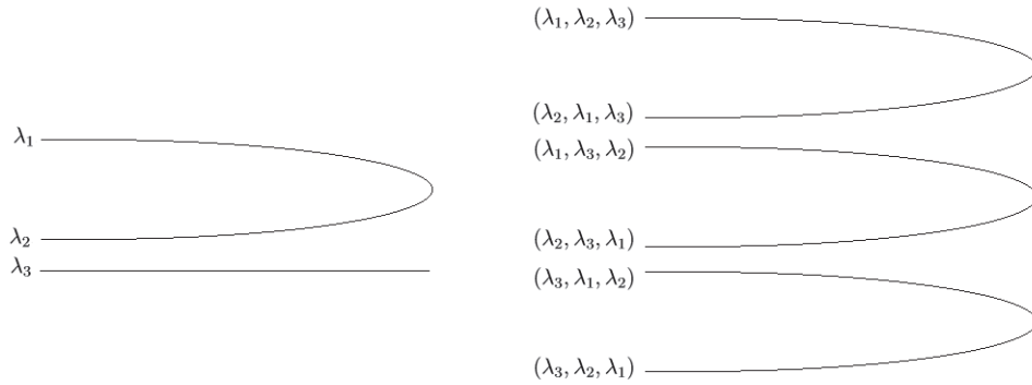
Figure 2.1: Preimage of a branch point of order 2, in the spectral (left) and cameral (right) curves.
