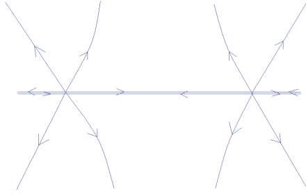
Figure 4.2: Saddle trajectory, cameral view.
