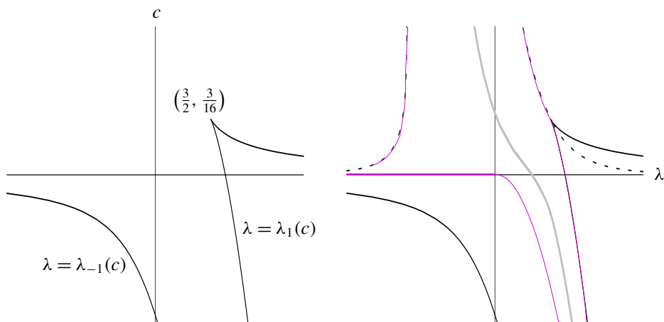
Figure 1. Left: Locus in parameter space where |\sin \psi| = 1 has a double root. Right: Numerically computed torus curve and region of parameter values possibly corresponding to tori (see page 288).
